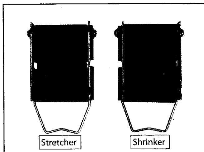
Figure 4. Assembled dies.
